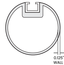
4" POST / CROSSBAR
