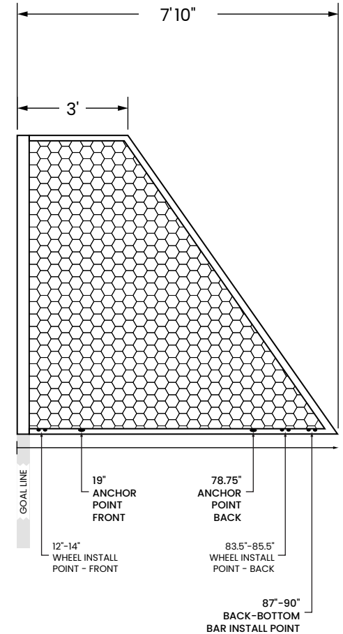
SIDE VIEW
